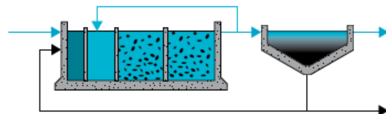
Hybas™ combination process with nitrification and pre-denitrification for nitrogen removal
